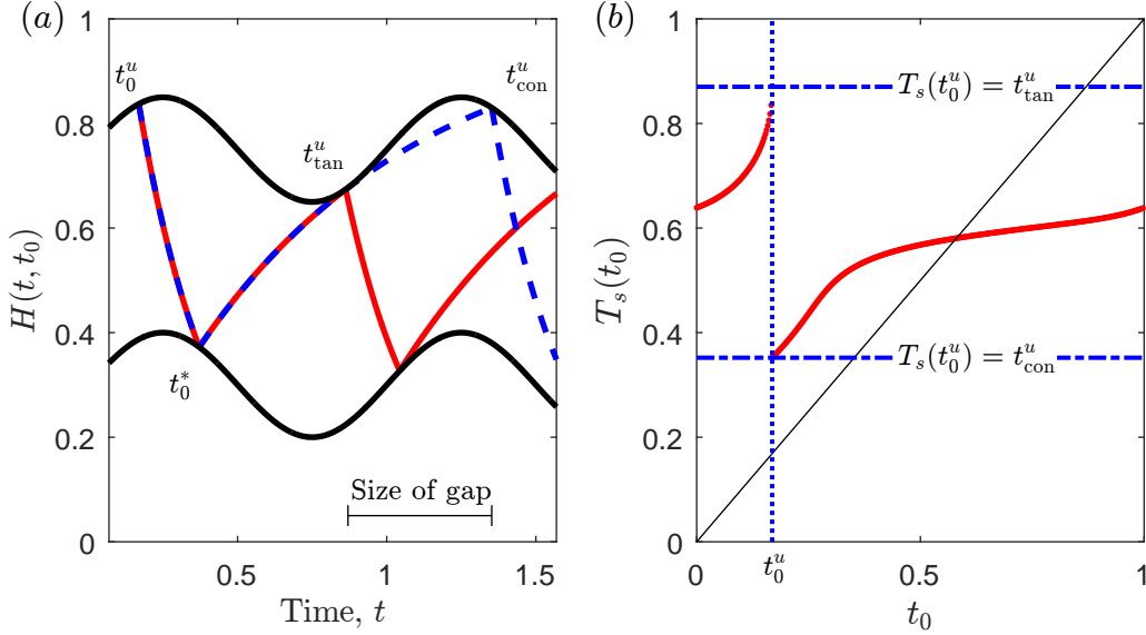
Figure 6. A small perturbation in start time t_0 can lead to large changes in the value of T_s(t_0) if, for t_0 , a tangency occurs between the homeostatic sleep pressure on sleep H_s(t) and the lower threshold, or the homeostatic sleep pressure on wake H_w(t) and the upper threshold. (a) Two possible trajectories with initial time t_0^u are shown. The bold red line shows the homeostatic sleep pressure switching at the tangency point H^+(t_{\text{tan}}^u) and dashed blue line shows the homeostatic sleep pressure missing the tangency and continuing on a wake trajectory; (b) The corresponding map shows the gap in T_s(t_0) occurring at t_0^u . Here we use a = 0.1 and H_0^- = 0.3 .
