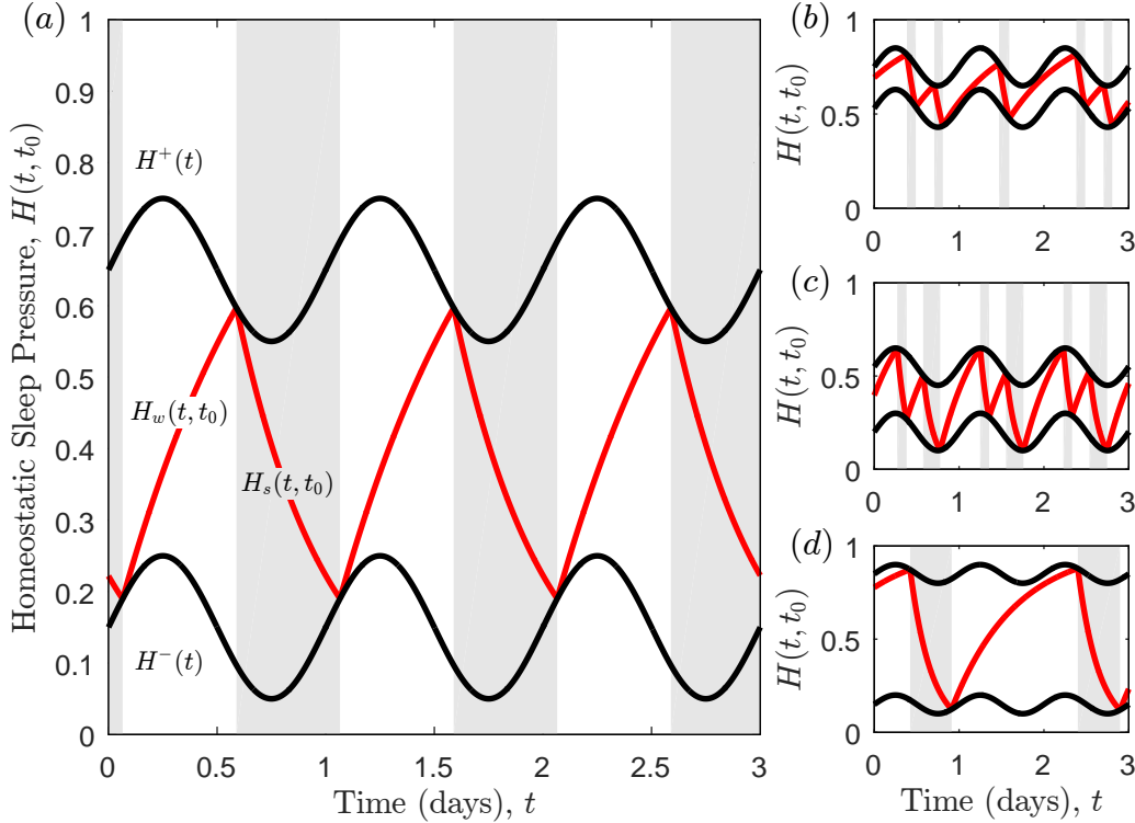
Figure 1. The two process model. (a) A one sleep/day periodic sleep-wake cycle, showing the homeostatic sleep pressure (shown in red) increasing during wake until it hits the upper threshold and then decreasing during sleep (shaded regions) until it hits the lower threshold. The thresholds are shown in black. Parameter values: a = 0.1, H_0^- = 0.15, H_0^+ = 0.65, \chi_s = 0.417, \chi_w = 0.75 . (b), (c) and (d) show three other possible patterns that occur as parameters are varied. Parameter values: (b) a = 0.1, H_0^- = 0.53, H_0^+ = 0.75, \chi_s = 0.25, \chi_w = 0.75 giving a sleep-wake cycle that repeats every two days with three sleep episodes; (c) a = 0.1, H_0^- = 0.2, H_0^+ = 0.55, \chi_s = 0.124, \chi_w = 0.5 giving a sleep-wake cycle that repeats every day with two sleep episodes; (d) a = 0.05, H_0^- = 0.15, H_0^+ = 0.85, \chi_s = 0.25, \chi_w = 0.75 giving a sleep-wake cycle that repeats every two days with one sleep episode.
