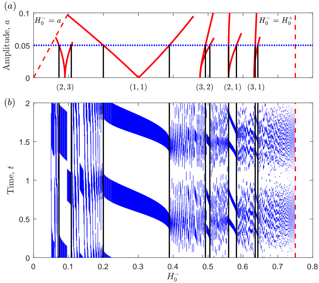
Figure 5. (a) Bifurcation set in the (H_0^-, a) -plane showing the largest few tongues where saddle node bifurcations give the boundary of each tongue. (b) Bifurcation diagram for a = 0.05 . Sleep-wake patterns associated with the \omega -limit set, plotted over two days for a dense grid of H_0^- values, with sleep plotted in blue. Black lines on panel (a) and on panel (b) have been drawn to help identify the boundaries of the Arnold tongues at a = 0.05 , given by the dashed blue line in (a).
