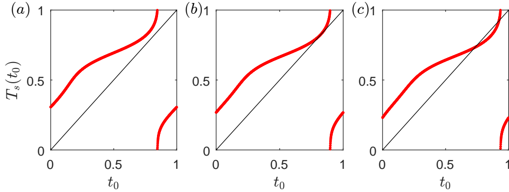
Figure 3. The creation of a pair of (p, q) = (1, 1) solutions via a saddle-node bifurcation for a = 0.05 and H_0^- varying. (a) No fixed points, H_0^- = 0.177 ; (b) at the saddle-node bifurcation, H_0^- = 0.197 ; (c) two fixed points, H_0^- = 0.217 . Note that for these parameter values, the primary effect of H_0^- is to shift the position of the map rather than change its gradient.
