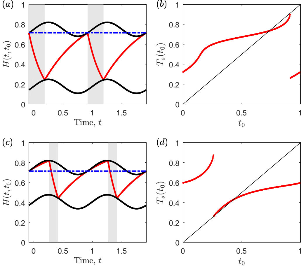
Figure 7. Type I and Type II border collisions of a (1, 1) periodic solution are shown for a = 0.07 . The dashed blue lines in (a) and (c) represent the value, H^+(t_{\text{tan}}^u) . (a) A sleep-wake cycle for a Type I border collision, switching from wake to sleep occurs at the time t_{\text{tan}}^u on the upper threshold; (b) The corresponding one-dimensional map shows the infinite derivative at the Type I border collision; (c) A sleep-wake cycle for a Type II border collision where the homeostatic sleep pressure on wake misses the upper threshold at H^+(t_{\text{tan}}^u) , switching at a later time (see Section 4.2); (d) The one-dimensional map for the Type II border collision. In (a,b) we have H_0^- = 0.178 and for (c,d) H_0^- = 0.4071 .
