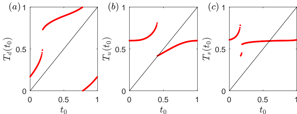
Figure 2. Typical examples of T_i \bmod 1 for i = d, u, s . Parameter values: a = 0.15, H_0^- = 0.25, H_0^+ = 0.75, \chi_s = 0.25, \chi_w = 0.75 . For the remainder of the examples in this paper we take H_0^+, \chi_s, \chi_w to be the values given here but a and H_0^- will vary.
