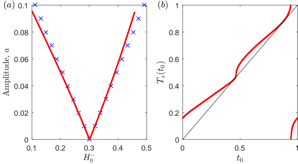
Figure 4. (a) A comparison of the numerical computation of the Arnold tongues for (p, q) = (1, 1) (solid lines) and the analytical expression for small a given in equation (3.7) (crosses). (b) The map of the two process model for a = 0.05 and H_0^- = 0.55 where a saddle-node bifurcation for the (2, 1) periodic solutions occurs.
