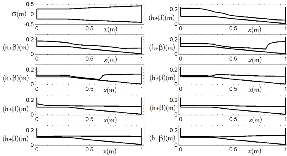
Figure 9: Sloshing inside an OWEL type vessel with prescribed surge forcing near dry states with FA5WS solver: first row from left to right: vessel cross-section versus x(m) and snapshot of the wave profile at t = .1 s . Second row from left to right: snapshots of the wave profile at t = .4 s and t = .7 s . Third row from left to right: snapshots of the wave profile at t = 1.1 s and t = 1.6 s . Fourth row from left to right: snapshots of the wave profile at t = 2.2 s and t = 3 s . Fifth row from left to right: snapshots of the wave profile at t = 3.5 s and t = 4 s .
