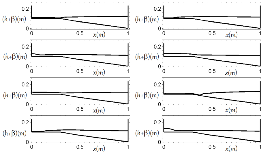
Figure 10: Continued: first row from left to right: snapshot of the wave profile at t = 4.6 s and t = 5.1 s . Second row from left to right: snapshots of the wave profile at t = 5.5 s and t = 6.3 s . Third row from left to right: snapshots of the wave profile at t = 7 s and t = 7.7 s . Fourth row from left to right: snapshots of the wave profile at t = 8.5 s and t = 9 s .
