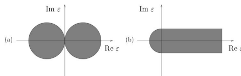
FIG. 13. (a) Region C_R in the complex \varepsilon -plane and (b) striplike region of analyticity S_B of the Borel transform. The region C_R is the union of two discs of radius R/2 and centers (\pm R/2, 0) .
