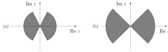
FIG. 15. Region \mathcal{D}_{R,\lambda} in the complex \epsilon -plane for \lambda = \tan \pi/6 (a) and for \lambda = 1 (b). One can write \lambda = \tan \varphi , where \varphi is the angle between the imaginary axis and the line a = \lambda b .
