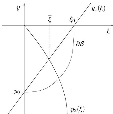
Fig. 1. Construction used in the proof of Lemma 3.
