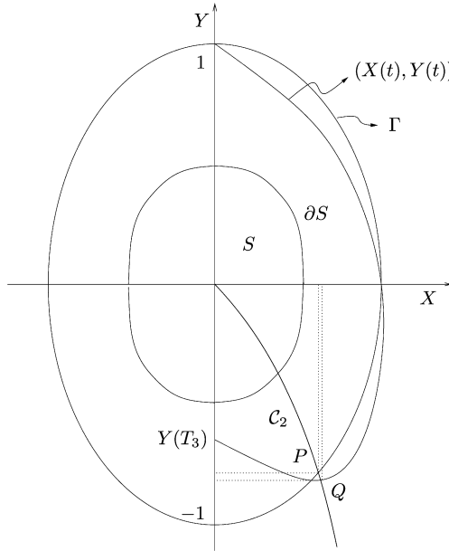
Fig. 3. Construction used in the proof of Lemma 5.
