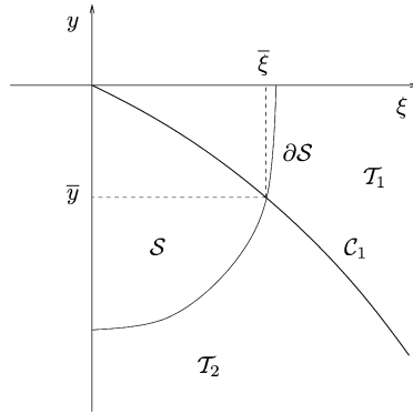
Fig. 2. Construction used in the proof of Lemma 4.
