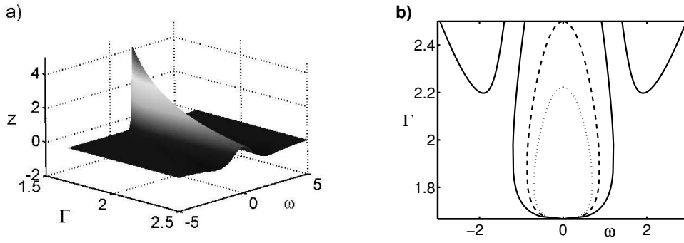
Figure 2. In both pictures 4(k + a) + v^2 = 5 . a) The plot of z(\omega, \Gamma) as defined by (32). b) The bounded regions in the \Gamma - \omega plane are the regions for which the perturbed invariant manifolds intersect transversely for \delta = 1 (dotted line), \delta = 2 (dashed line) and \delta = 10 (solid line).
