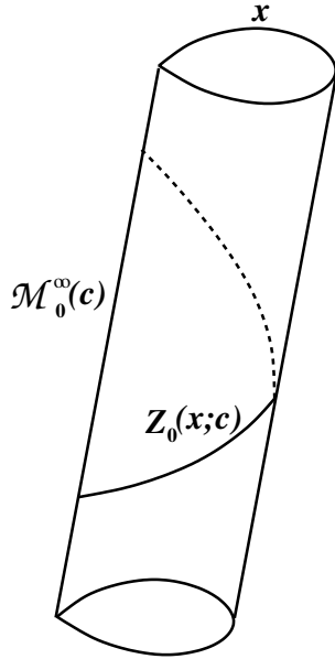
Figure 1. Geometry of the invariant two-dimensional manifold \mathcal{M}_0(c) of the unperturbed system for a fixed value c \in \mathcal{C} . Different points on the group orbit G_\theta Z_0^\infty(c) are connected by the relative heteroclinic orbits Z_0(x; c) .
