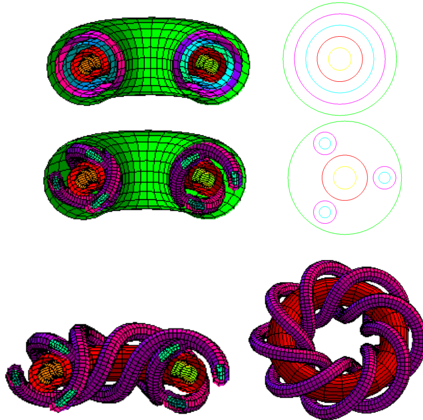
Fig. 7: Top: five tori before perturbation (we denote the green, red and yellow tori as irrational and the purple and blue tori as rational) with cross-section; Middle: the five tori after perturbation (the purple and blue tubes replace the tori) with cross-section; Bottom Left: stripping away the outer torus shows the tube-like objects; Bottom Right: full view of the purple tube wound around the red torus.
