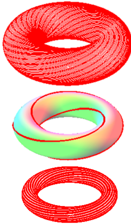
Fig. 4: Rational orbit with p = 2 and q = 3 (Middle, radius is l_B ) and two irrational orbits (Top and Bottom, radii are l_A and l_C respectively); l_A > l_B > l_C .
