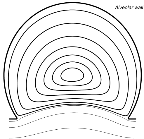
Fig. 1: Schematic of the recirculating alveolar flow pattern calculated in an asymmetric alveolar duct model, which is driven by flow past the alveolar entrance [modified from Tsuda et al., 1995].
