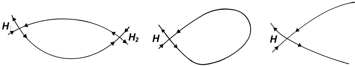
Fig.10: These are the possible scenarios for integrable Hamiltonian systems – curves with arrows pointing towards H are stable, those pointing out are unstable; Left: heteroclinic orbit (or heteroclinic connection); Middle: homoclinic orbit (or homoclinic connection); Right: the curves lead off to infinity.
