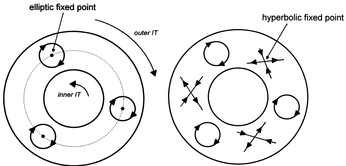
Fig. 8: Left: the direction of closed curves – solid outer and inner circles are from irrational tori (IT) and the dotted circle comes from a rational torus; Right: in between the circles that surround elliptic fixed points, other points must exist to balance the direction of movement (of particles) – the points lying at the center of the crosses are hyperbolic fixed points.
